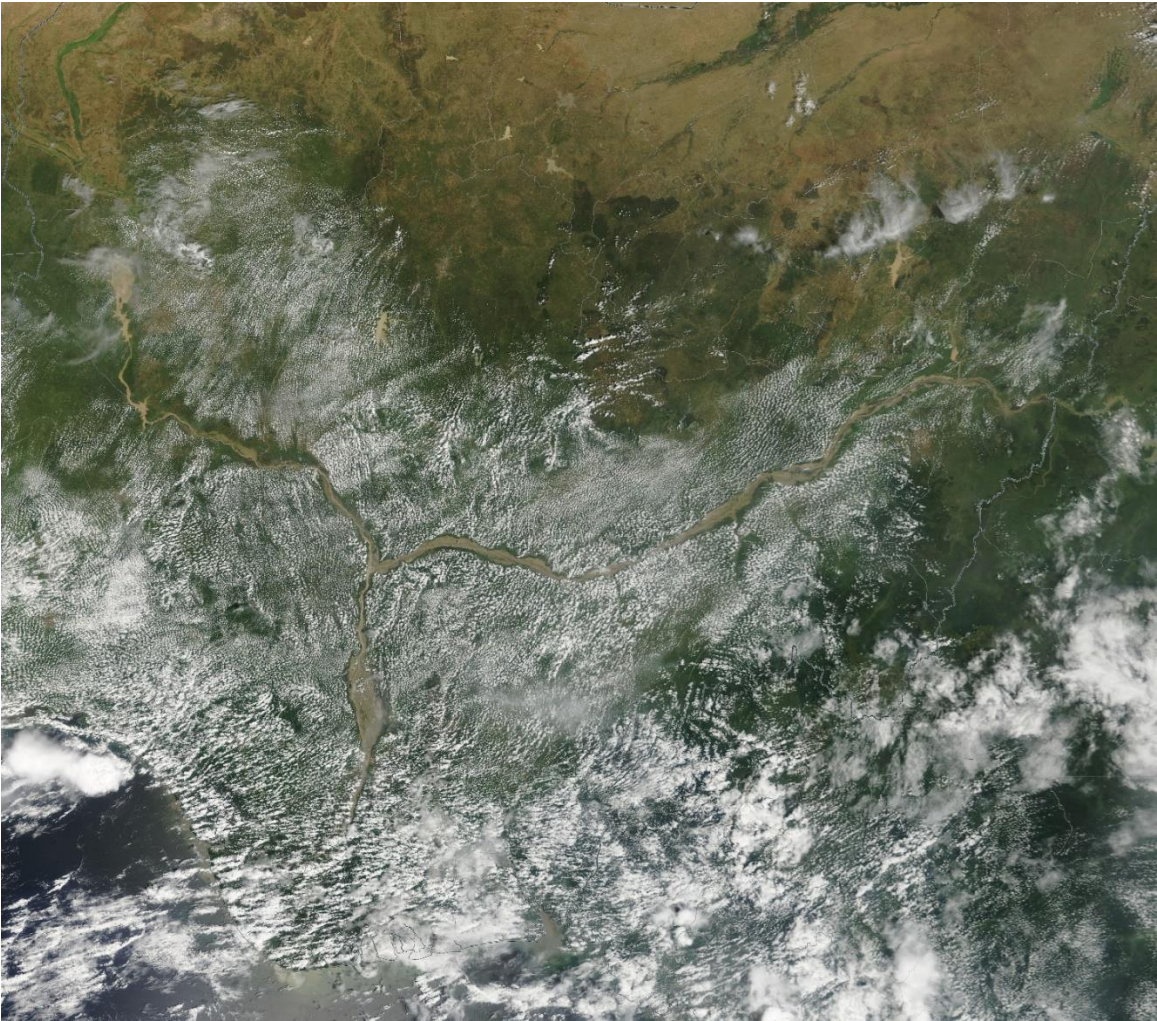
Figure A 6: Terra MODIS True Color Corrected Reflectance snapshot 13 October 2012
